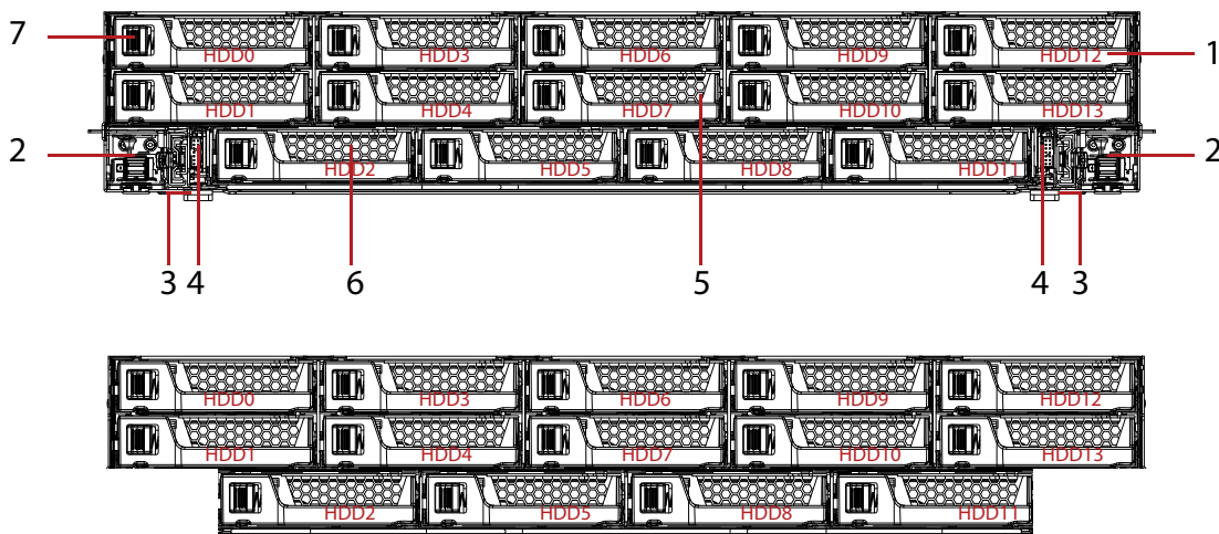
Figure 1-1. System Front View
