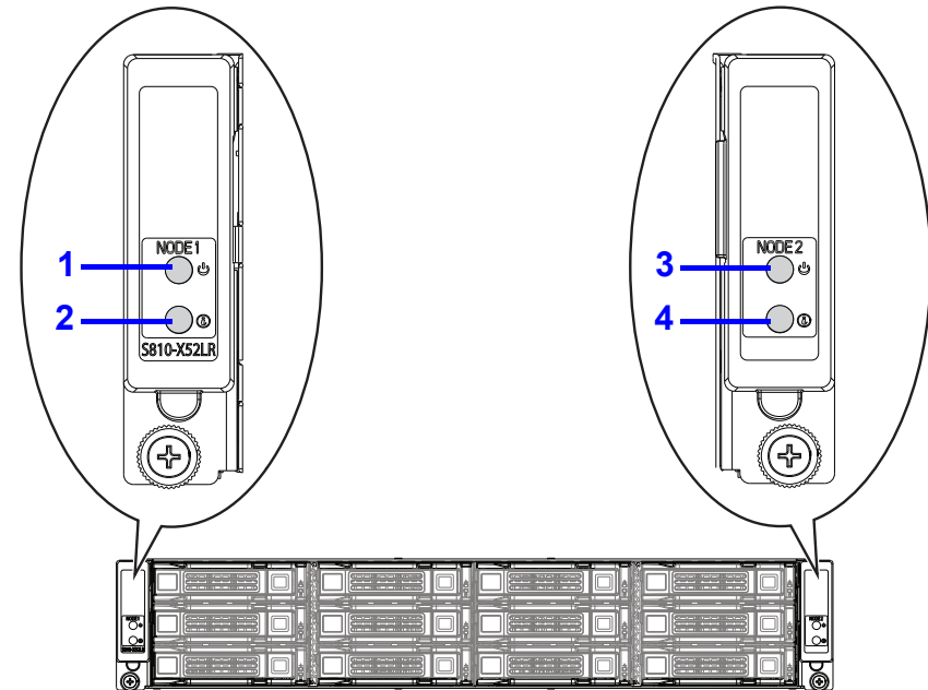
Node Front Panel Features
