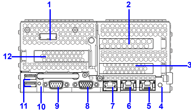
System Rear I/O Features (Configuration 2)
