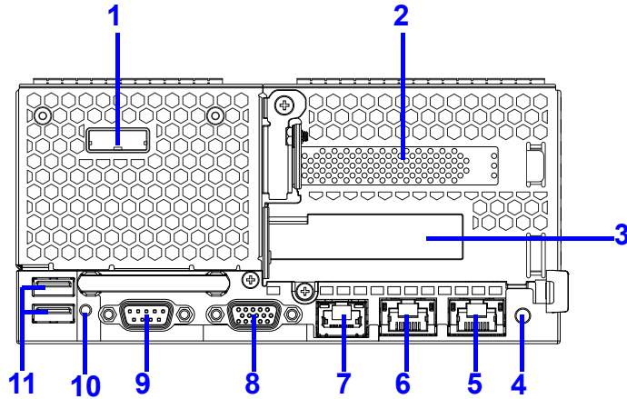
System Rear I/O Features (Configuration 1)
