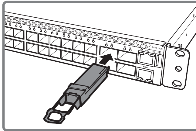
Figure 3-9: Connect QSFP+ Module
