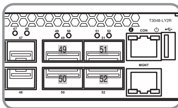
Figure 3-8: QSFP+ Port Numbering
