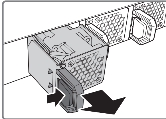
Figure 5-3: Remove Hot-swappable Fan Module
