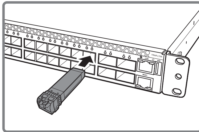
Figure 3-7: Connect SFP+ Module
