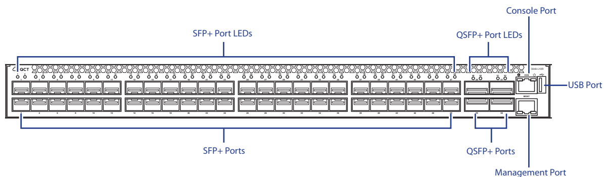
Figure 2-1: Front Panel View
