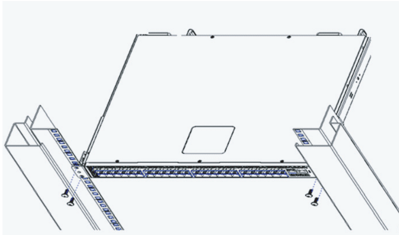
Figure 3-1: Install Switch on Rack (Without Rail)
